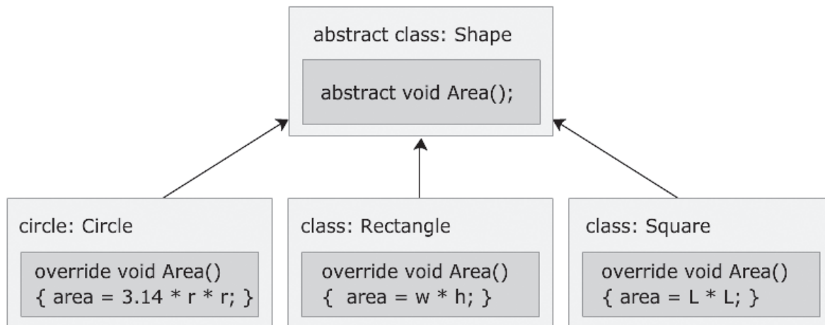
Figure 8.3: Abstract Class and Abstract Method
