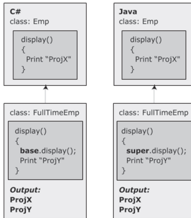
Figure 8.2: Calling Parent Class Method from Child Class Overridden Method
