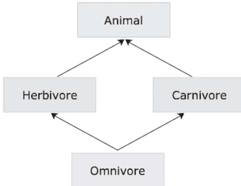
Figure 5.4: The Diamond Problem
