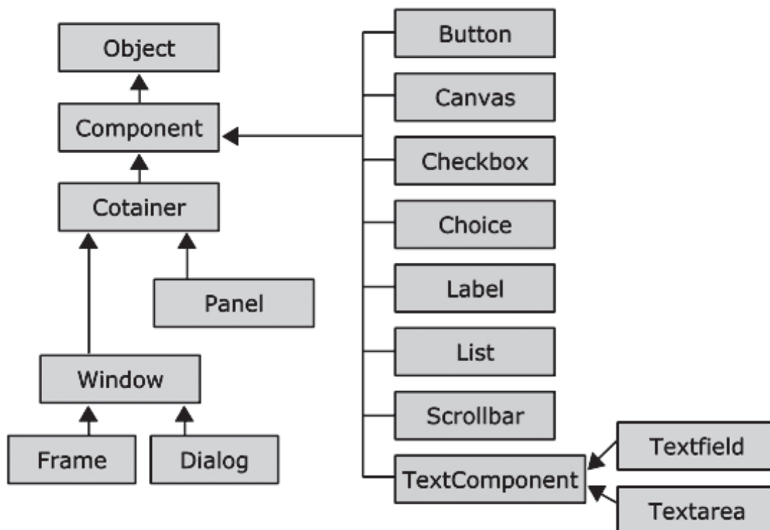
Figure 11.3: AWT Class Hierarchy
