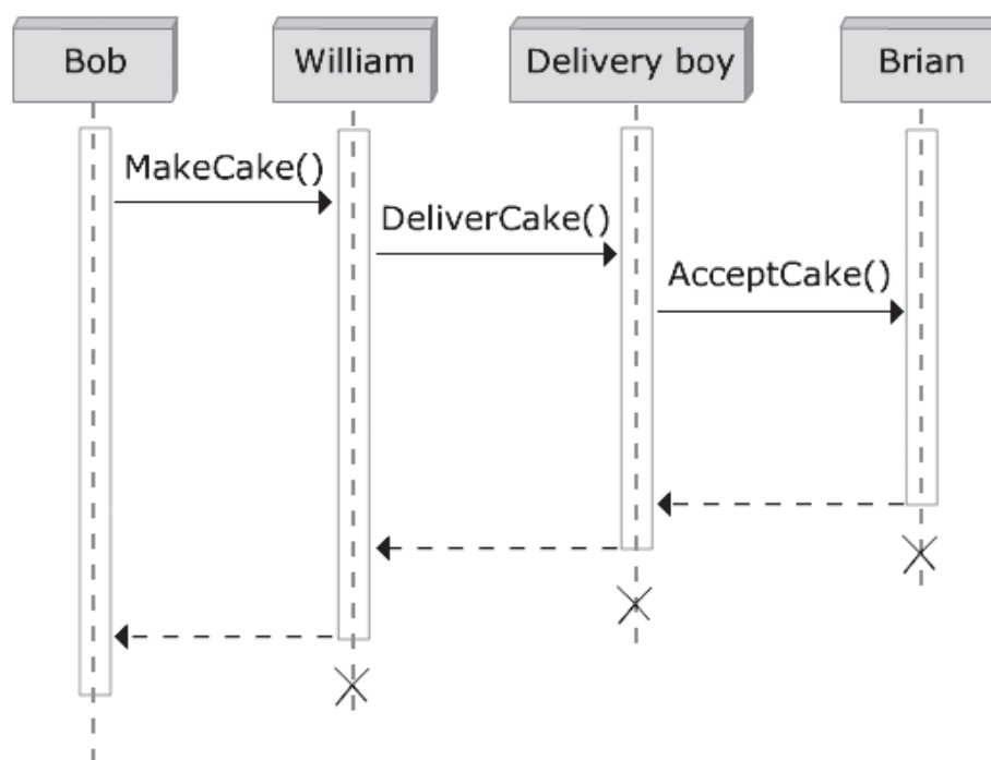
Figure 2.6: Method Invocation Amongst Objects in the Cake Delivery Process
