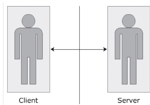
Figure 4.5: Level 3 Abstraction
