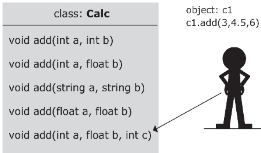
Figure 7.2: Method Overloading
