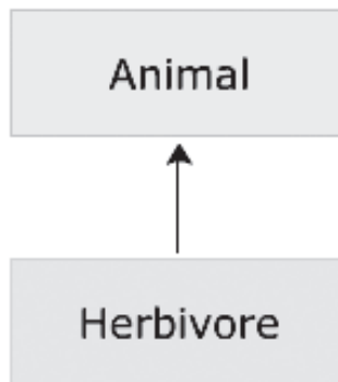
Figure 4.9: Single Inheritance
