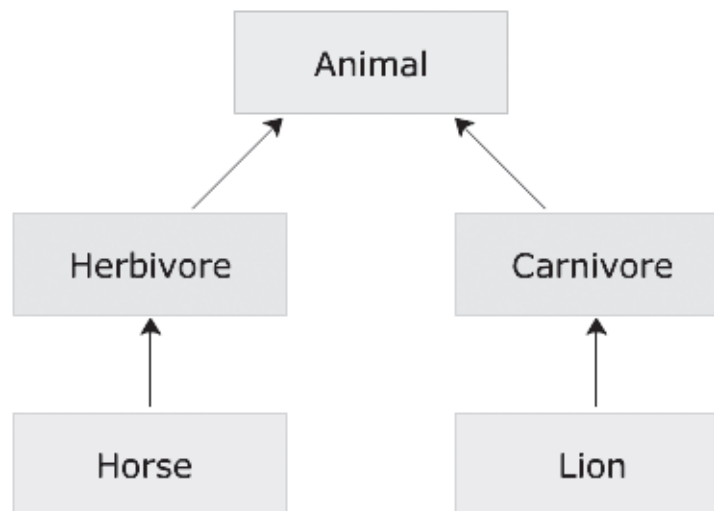
Figure 4.8: Inheritance
