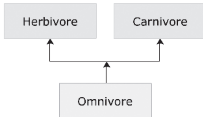
Figure 5.2: Multiple Inheritance
