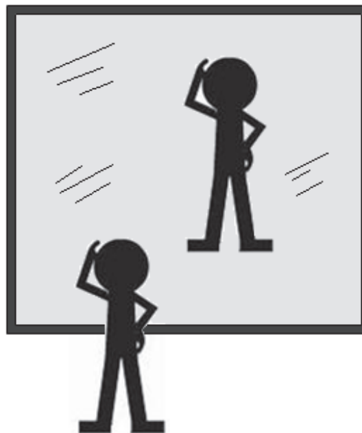
Figure 11.6: Reflection
