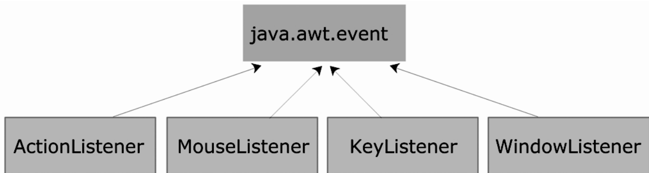
Figure 11.5: Event Listeners
