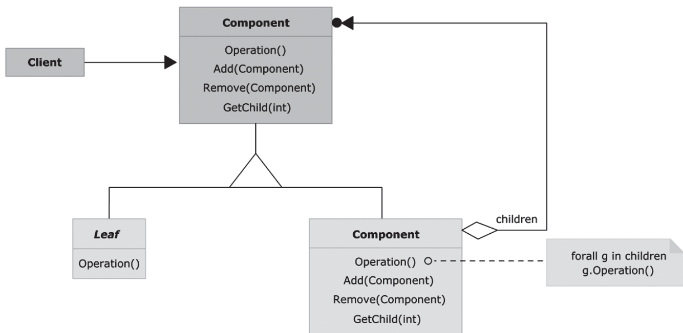
Figure 12.3: Class Diagram of Composite Pattern
