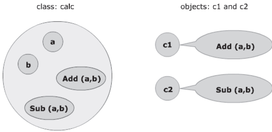
Figure 1.3: Encapsulation
