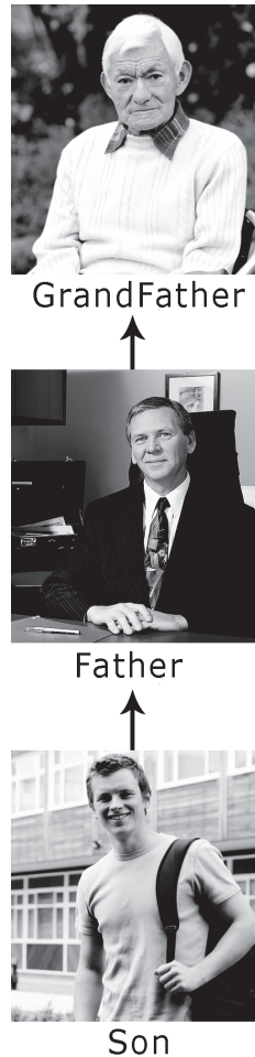
Figure 1.5: Inheritance
