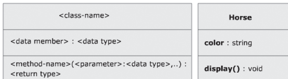
Figure 3.3: Class Diagram
