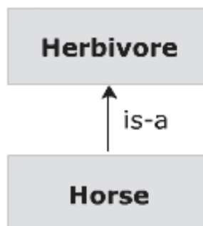
Figure 4.7: Is-a Abstraction
