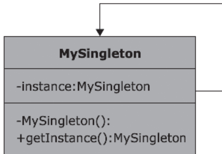
Figure 12.2: Singleton Pattern
