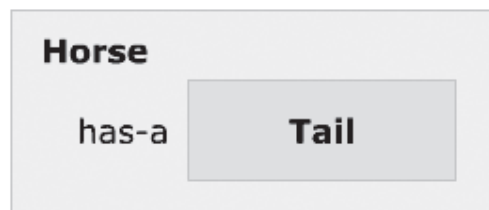
Figure 4.6: Has-a Abstraction
