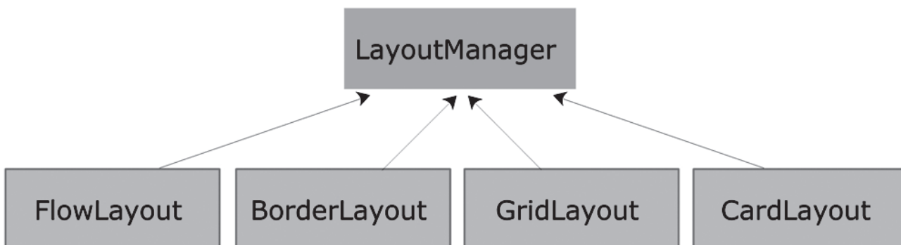
Figure 11.4: Layout Manager
