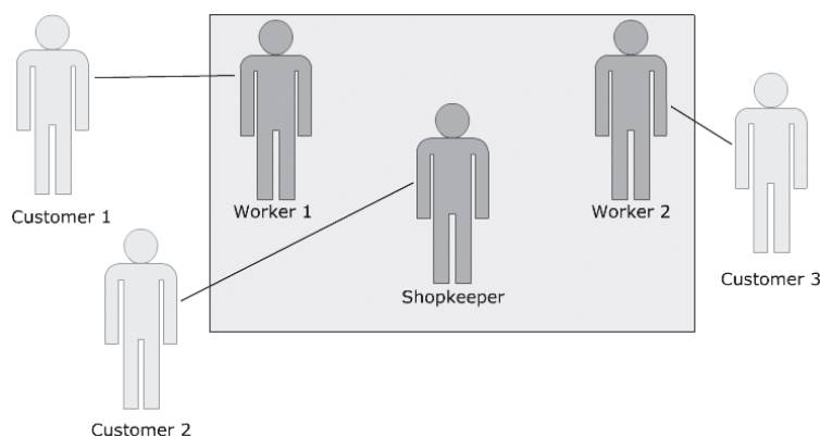
Figure 2.13: High Cohesion
