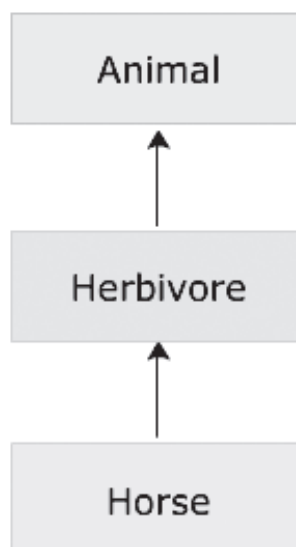
Figure 4.10: Multilevel Inheritance
