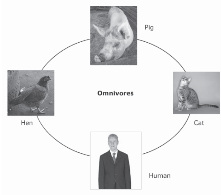
Figure 5.1: Omnivorous Animals
