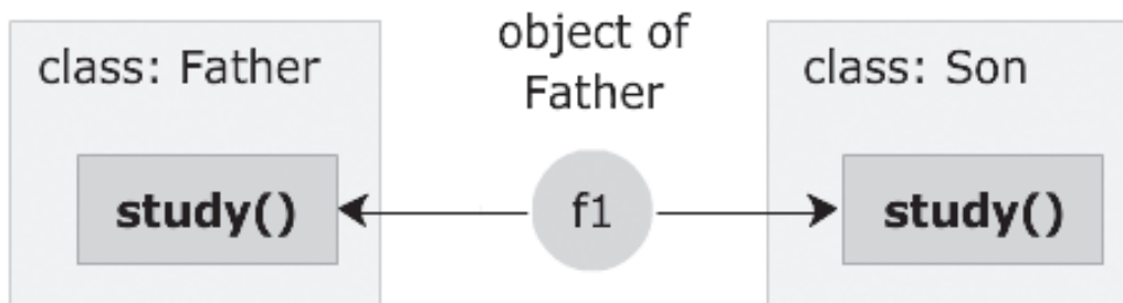
Figure 9.2: Polymorphic Variable
