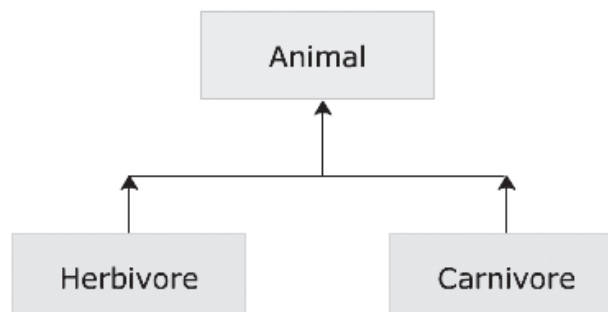
Figure 4.12: Hierarchical Inheritance
