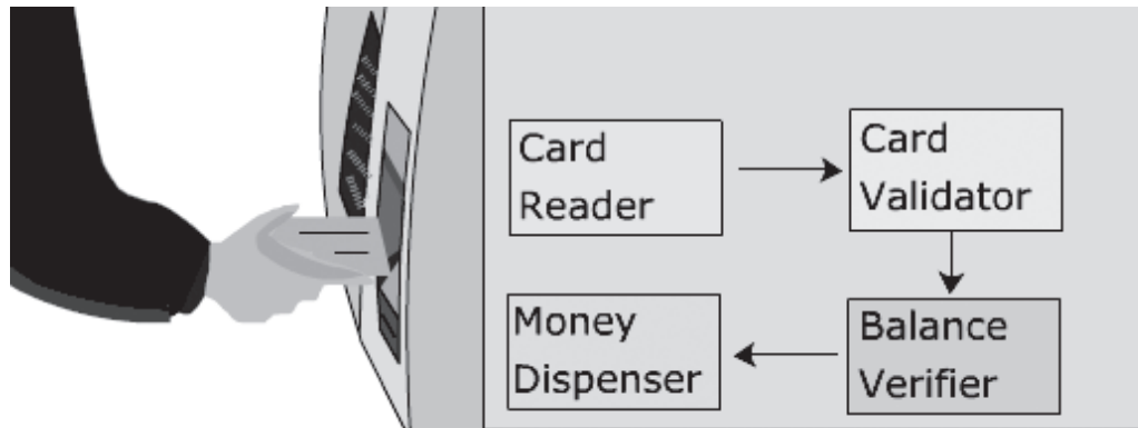
Figure 1.4: Abstraction
