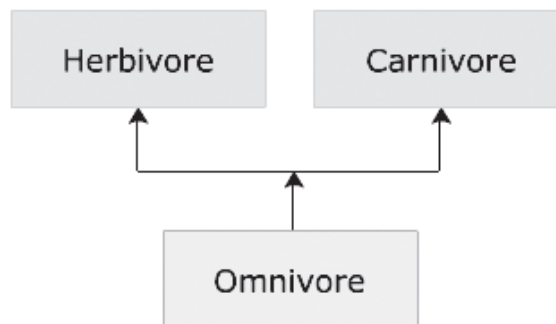
Figure 4.11: Multiple Inheritance
