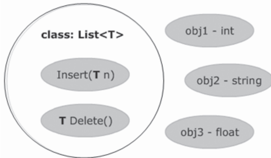
Figure 10.1: Generics
