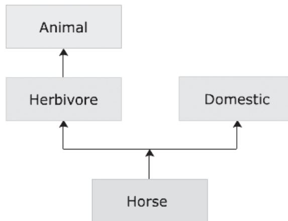
Figure 4.13: Hybrid Inheritance
