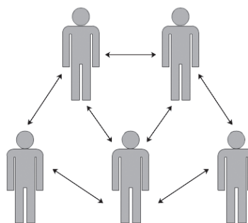
Figure 4.3: Level 1 Abstraction
