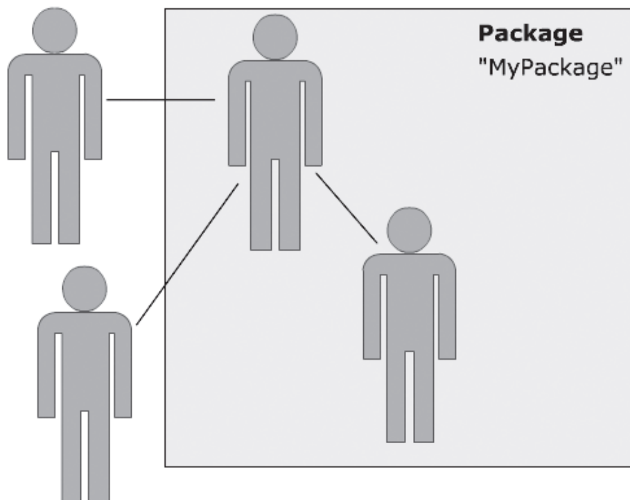
Figure 4.4: Level 2 Abstraction
