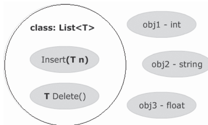
Figure 6.6: Generics
