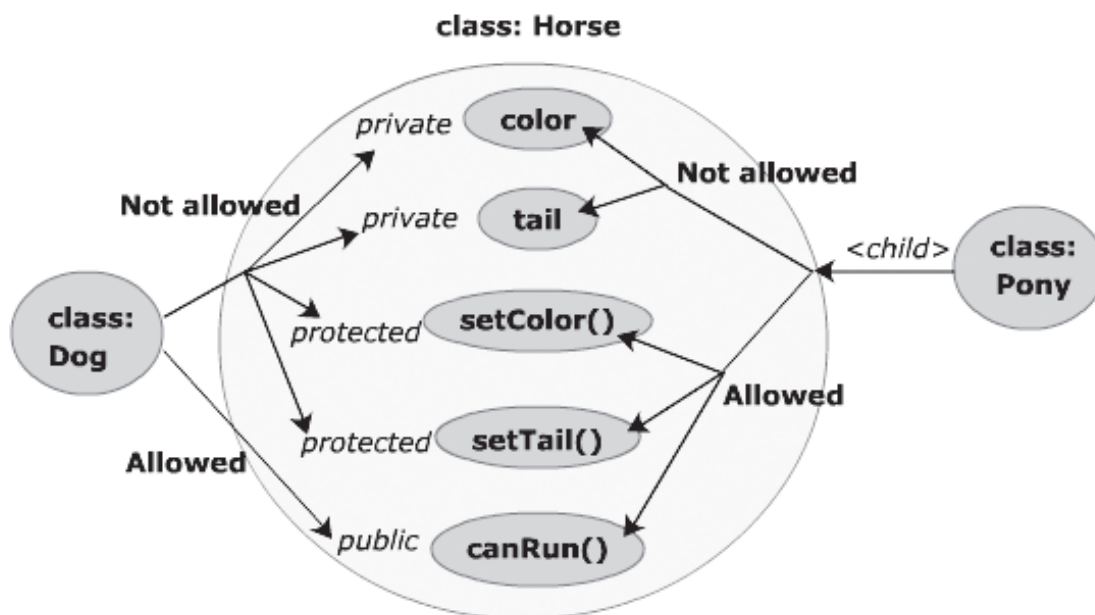
Figure 3.4: Visibility Modifiers
