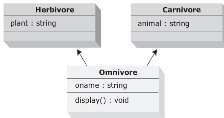
Figure 5.3: Class Diagram of Multiple Inheritance
