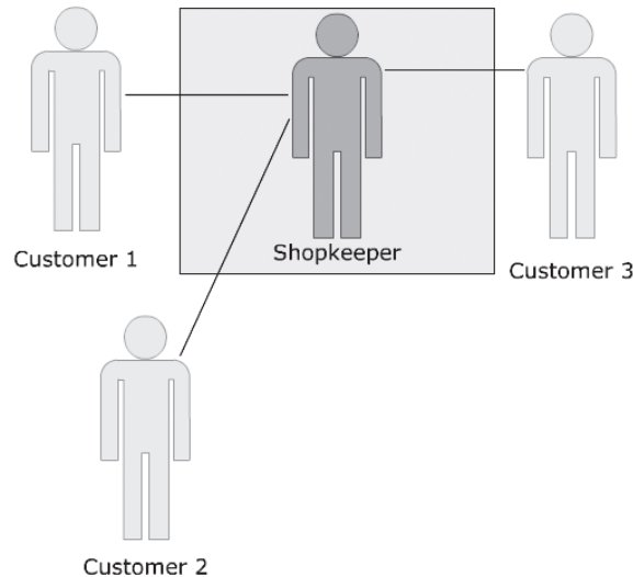
Figure 2.12: Low Cohesion
