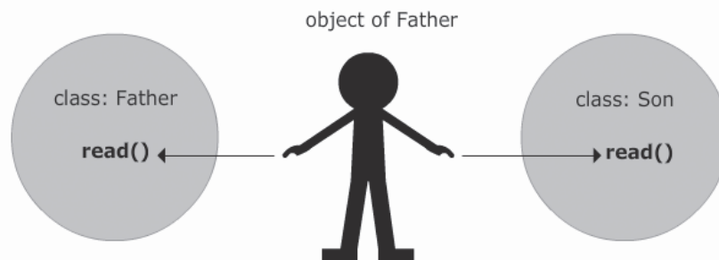
Figure 6.5: Polymorphic Variable
